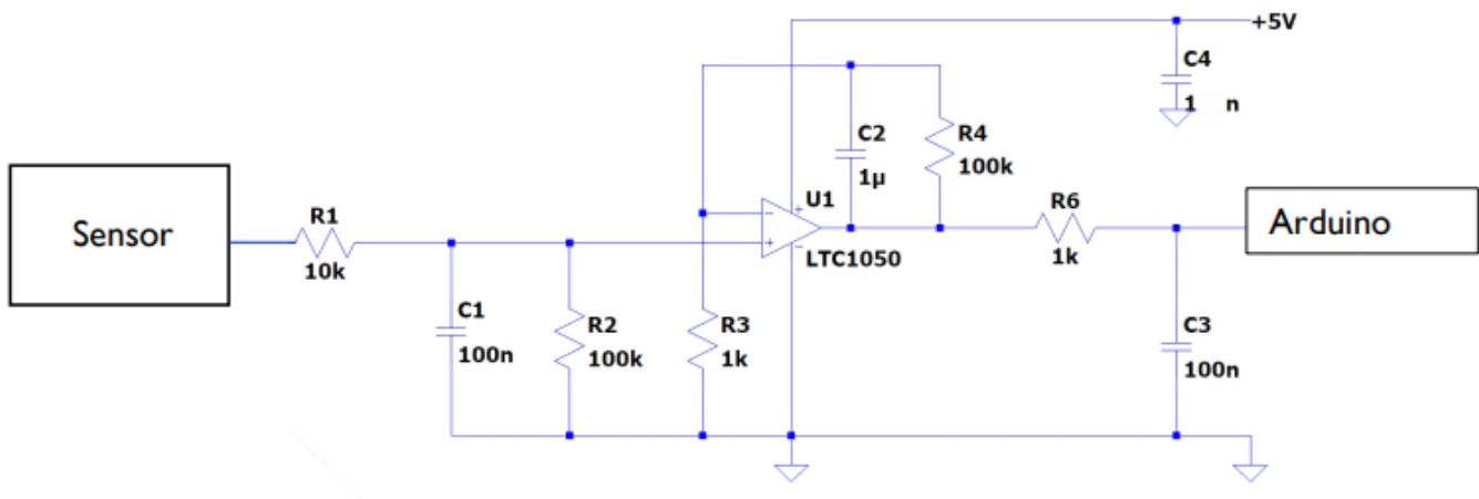
Figure 4: Proposed amplification circuit for measuring the signal
